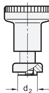
销头缩回状态 (如果 l_1 = d_1 )
